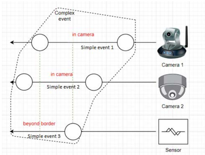
Fig. 6. A space-time graph of an event
