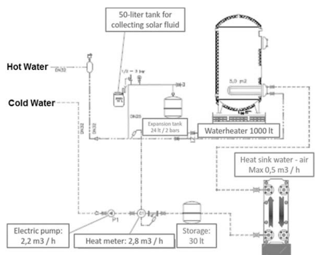
Fig.3. Schematic View Of The Auxiliary Hydraulic Components In-Out The Module
