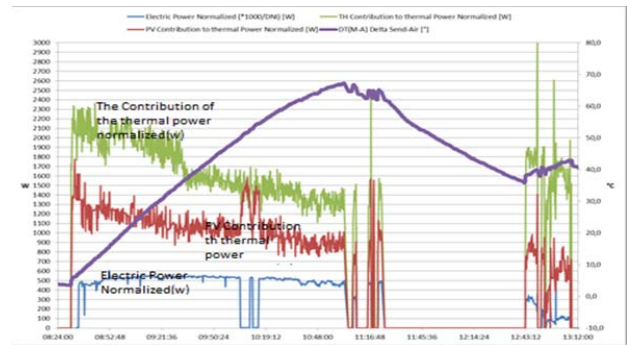
Fig.4. show the performance of the system and the production of electrical and thermal power
