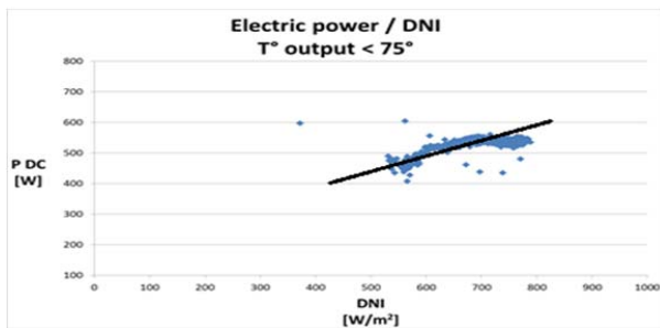
Fig.6. the Output Power with Respect to DNI in W/m^2 at 75°C
