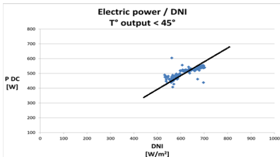
Fig.5. Output power with respect to DNI in W/m^2 at 45°C
