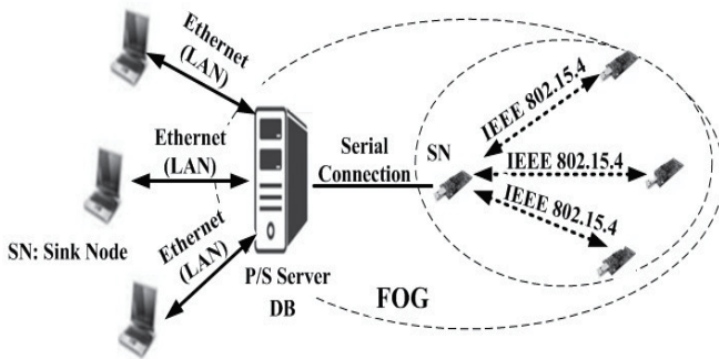
Fig. 3. Testbed setup
