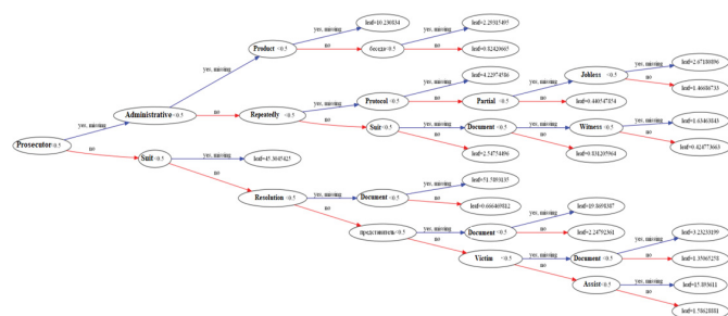
Fig. 3. Regression tree for the administrative and criminal ruling
